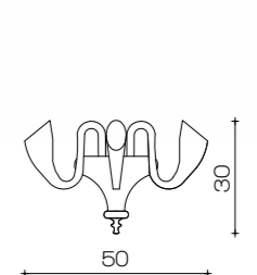
Art.1965/A3 H 30 cm ø 50 cm 3 x G9 X 40W
