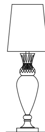
Art.1953/P H 82 cm Pø 26 cm 1 x E27 x 40W
