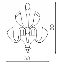
Art.1965/A6 H 60 cm ø 50 cm 6 x G9 X 40W
