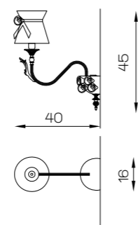
Art.1850/A1 H 45 cm Pø 16 cm Sp 40 cm 1 x E14 x 40W
