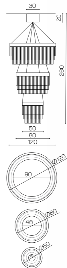
Art.1972 H 260 cm ø 120 cm + Ceiling plate H 20 cm ø 30 cm with 3 spot Led (5W 450 LUMEN) + Strip Led Colour light 2700°K Lumen 16530
