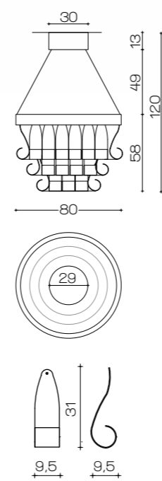
Art. 1937 Chandelier H 58 cm ø 80 cm + Ceiling plate H 13 cm ø 30 cm with 3 spot Led (5W 450 LUMEN) H tot. 120 cm + Strip Led Colour light 2700 K° Lumen 8550
