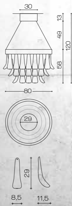
Art. 1939 Chandelier H 58 cm ø 80 cm + Ceiling plate H 13 cm ø 30 cm with 3 spot Led (5W 450 LUMEN) H tot. 120 cm + Strip Led Colour light 2700 K° Lumen 8550
